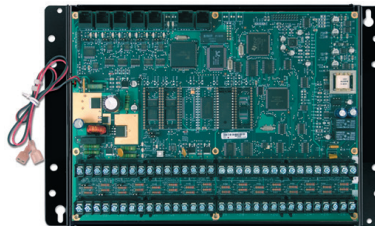
20A00-52 Omni IIe for Structured Wiring Enclosures
